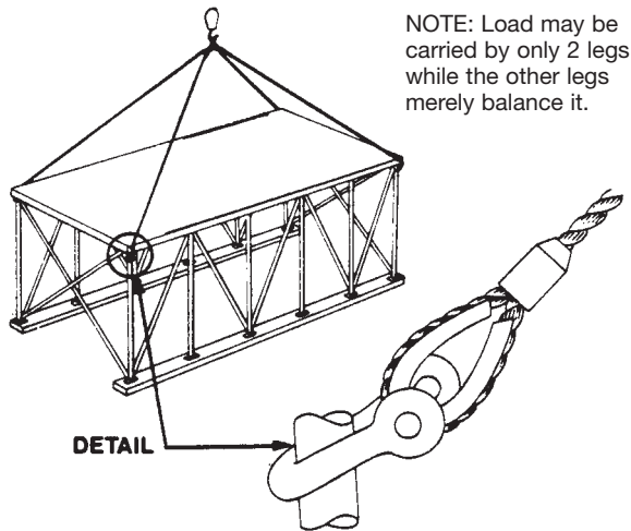
4-LEG BRIDLES HITCH Figure 13
